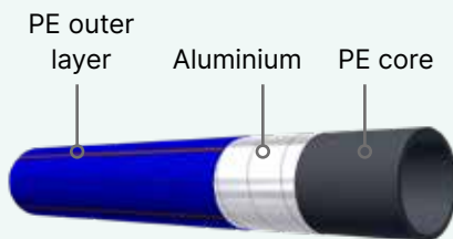
Puriton® pipe structure
