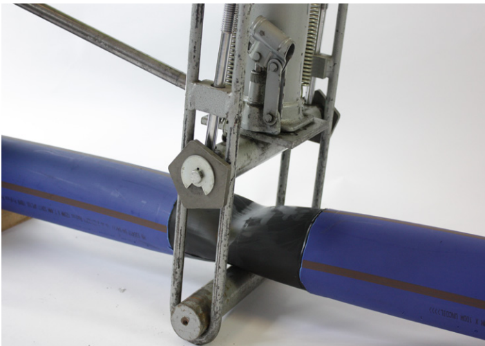
Fig 8. Tool fully open ready for removal
