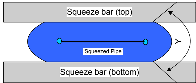
Fig 5. Sectional view through a squeezed off pipe Y = 4 \times \text{pipe wall thickness} .
