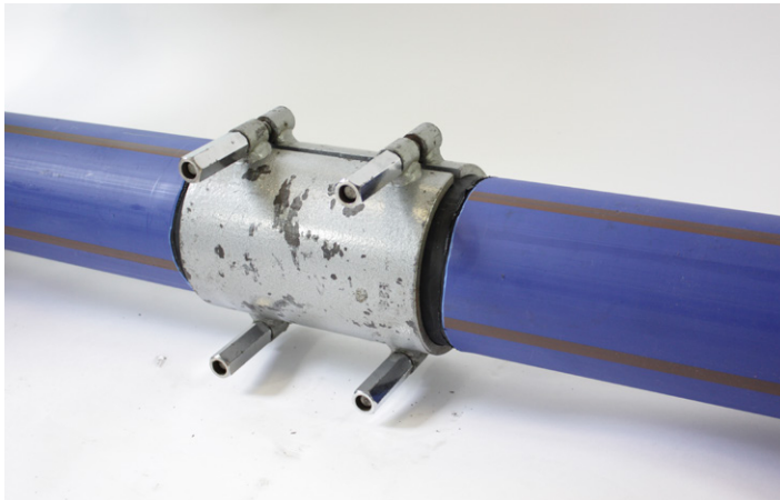
Fig 9. Mechanical re-rounding clamp in position on the pipe over the squeeze off location
